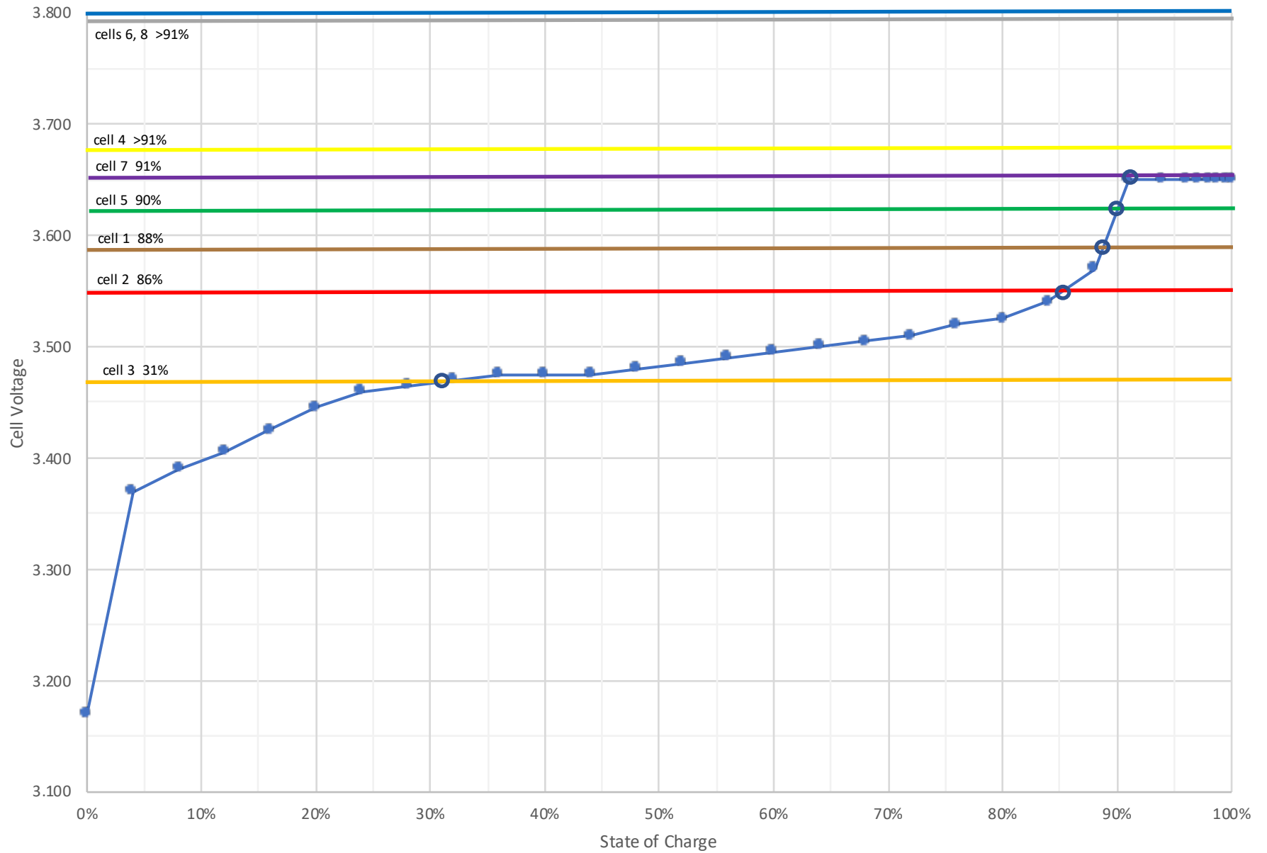
LiFePO4 Cell Voltage vs. State of Charge - e-Mower Charge #1, 4/3-4/2020
