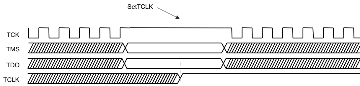
Figure 2-6. SetTCLK
