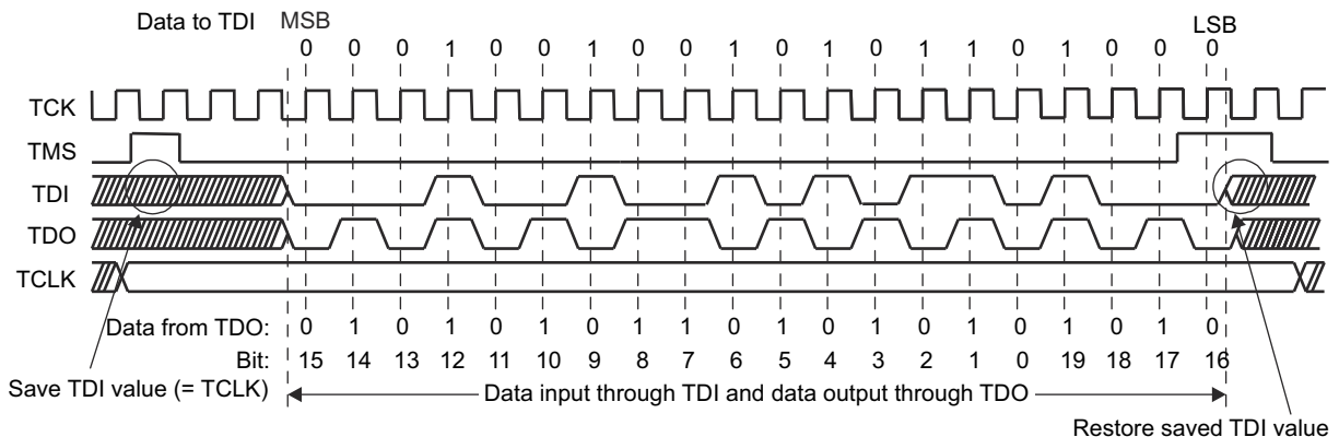
Figure 2-5. Address Register I/O: DR_SHIFT20 (0x12568) (TDO Output Is 0xA5AA)
